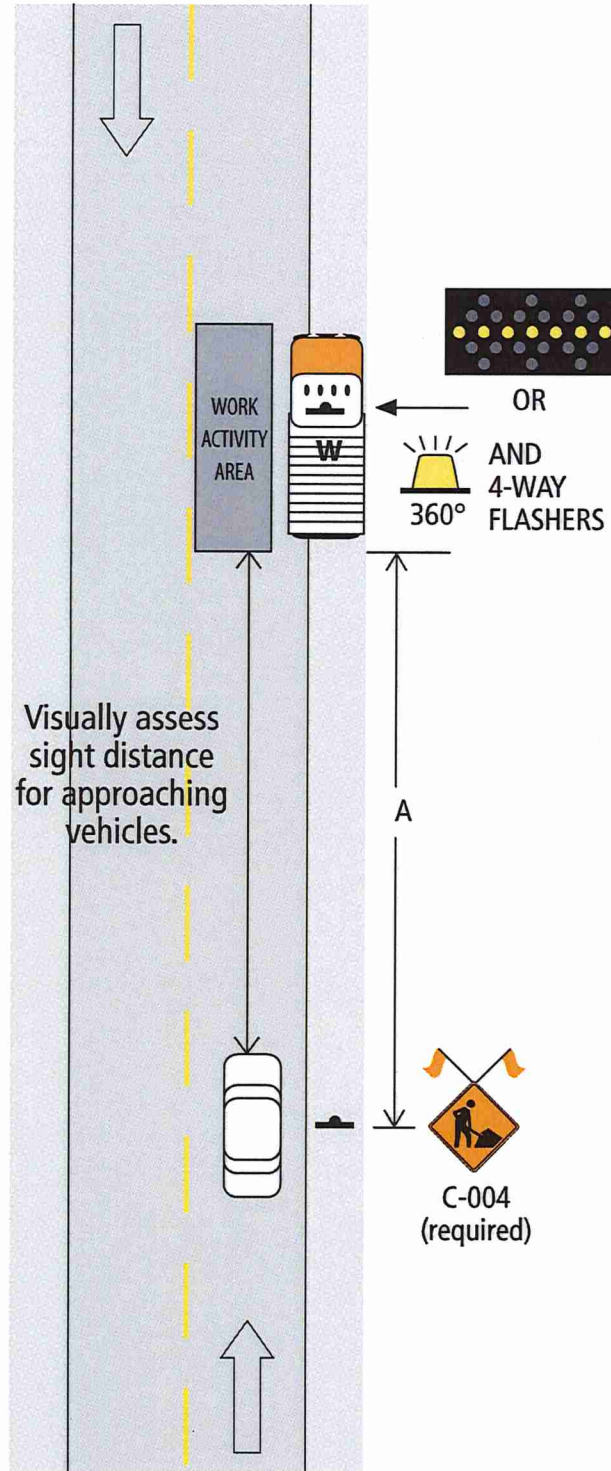
Figure 7.4: Brief-Duration Work – Two-Lane, Two-Way Roadway
